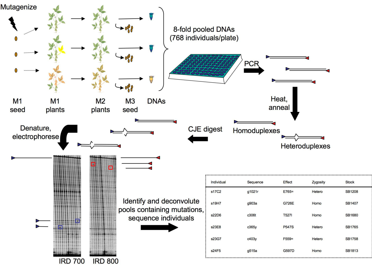
Figure 1 Schematic of the soybean TILLING process [39]. Seeds are mutagenized and grown to generate the M1. Since the embryo consists of many cells, M1s may be mosaic for mutations induced by the mutagen. M1 plants are allowed to self and a single M2 plant is grown from each M1 line. Tissue and M3 seed are collected from the M2 plants. The concentration of DNAs isolated from the M2 tissue is normalized, and the samples are pooled eight-fold in 96-well plates. IRDye labeled primers are used for amplification of a particular target. Following PCR, samples are denatured and allowed to reanneal such that if a mutation is present, heteroduplexes will form. CJE is used to cleave 3' of the mismatch. Samples are denatured and electrophoresed on polyacrylamide gels using LI-COR 4200 or 4300 machines. Putative mutations are identified by bands appearing in the 700 and 800 channels that add up to the molecular weight of the full length PCR product. Pools are deconvoluted to identify mutant individuals, and the individuals are sequenced. Sample soybean gel section and complete results from the gmclavb primer set screened on the A population are shown.
